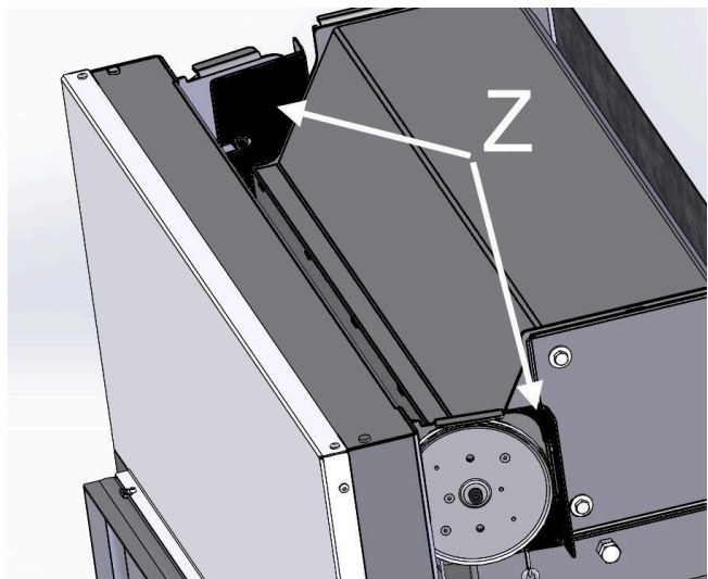
Im. 3: Installing of the heat protection shields
