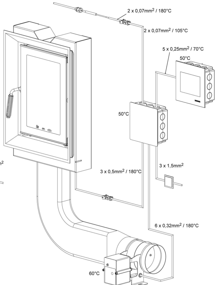
Im. 5: Schematic layout of EOS
