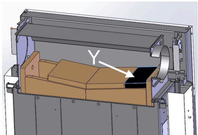
Im. 2: How to place the vermiculite plates
