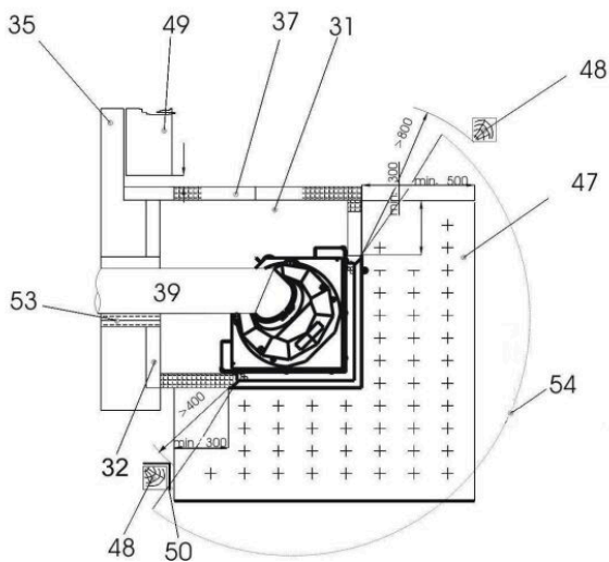
Im. 6: Basic principles of fire safety and heat insulation
