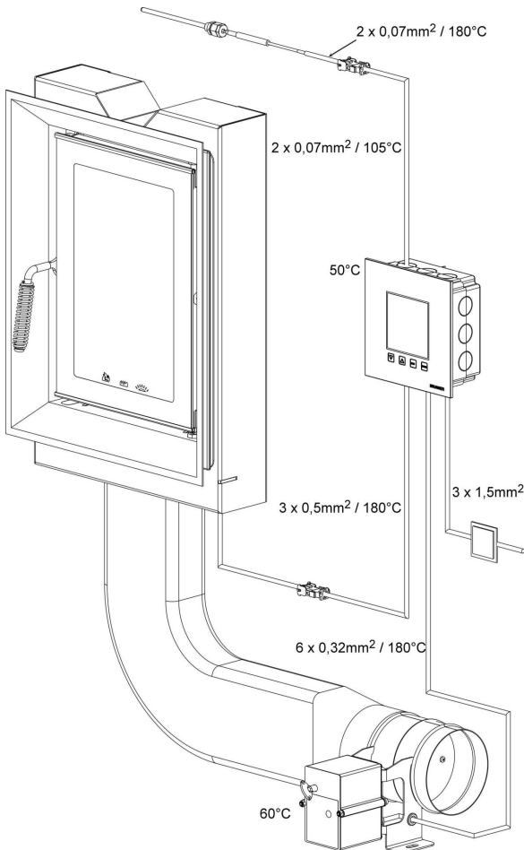
Im. 4: Schematic layout of EAS
